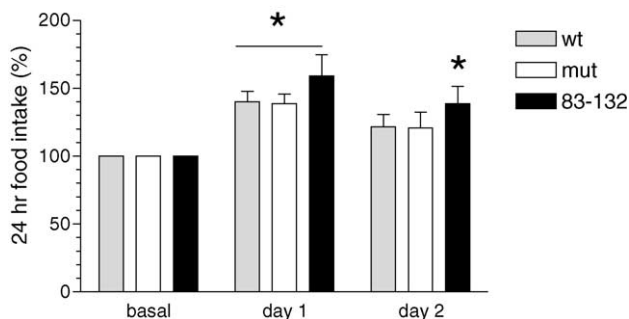
Fig. 6. Daily food intake of rats prior to and on two days following ICV injection of 1 nmol His-tagged Ala67 (wt; gray bar, n = 3) or Thr67 (mut; white bar, n = 4) full-length AgRP or AgRP 83–132 (83–132, black bar, n = 8) (mean \pm SEM; (*) significantly different from basal food intake; paired t -test; p < 0.05).
